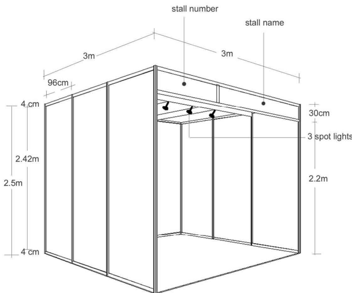
single side open stand
