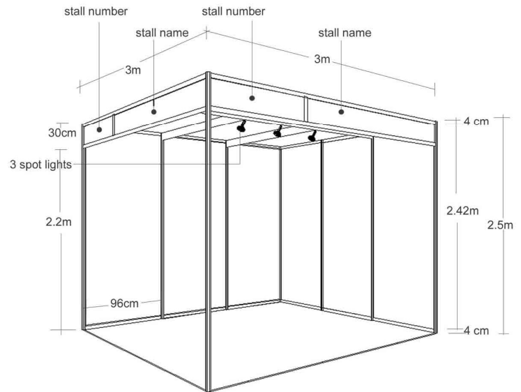
two side open stand
